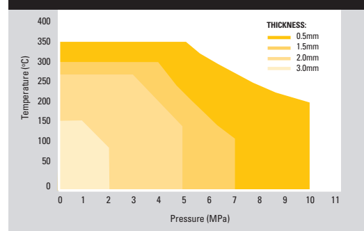
SF 3100 – PRESSURE / TEMPERATURE LIMITS
